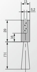
FBL 1340
