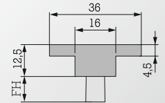
FBL 1340
