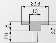
FBL 1330
